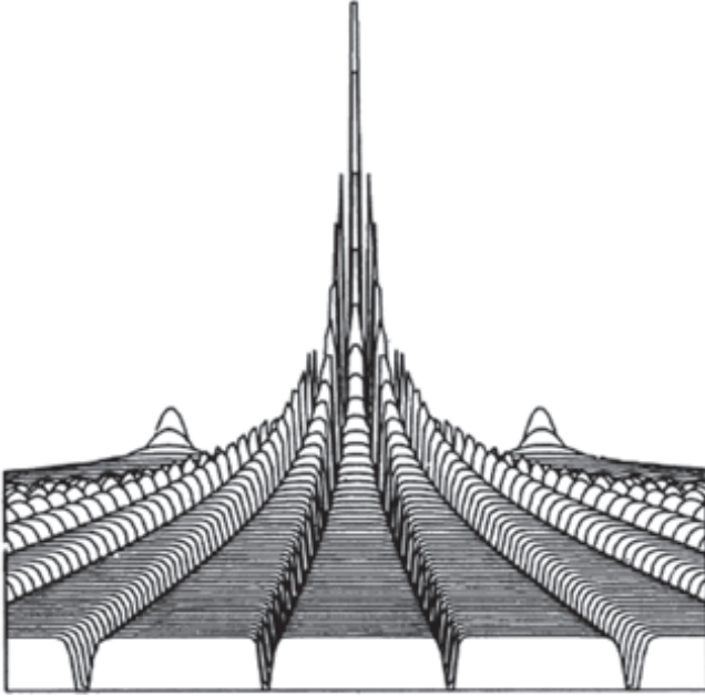
Figure 16.1 Quantum Potential for Two Gaussian Slits (from Philippidis, Dewdney and Hiley 1979). Reprinted with kind permission of Società Italiana di Fisica, copyright (1979) by the Italian Physical Society ( https://link.springer.com/article/10.1007%2FBF02743566 )
