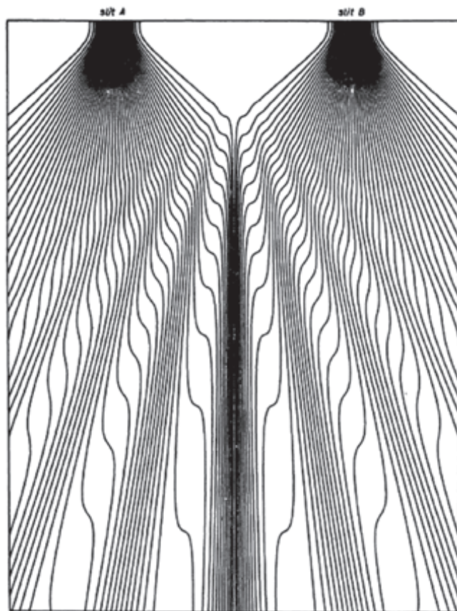
Figure 16.2 Trajectories for Two Gaussian Slits (from Philippidis, Dewdney and Hiley 1979) with kind permission of Società Italiana di Fisica, copyright (1979) by the Italian Physical Society ( https://link.springer.com/article/10.1007%2FBF02743566 )
